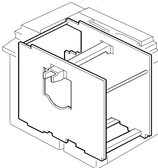
4.FRAME SECTION 2 (C228)
