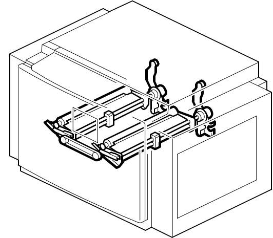
9. Pressure Roller Section 1 (C639)
