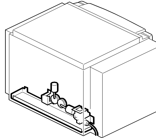
18. Drive Section 5 (C593)
